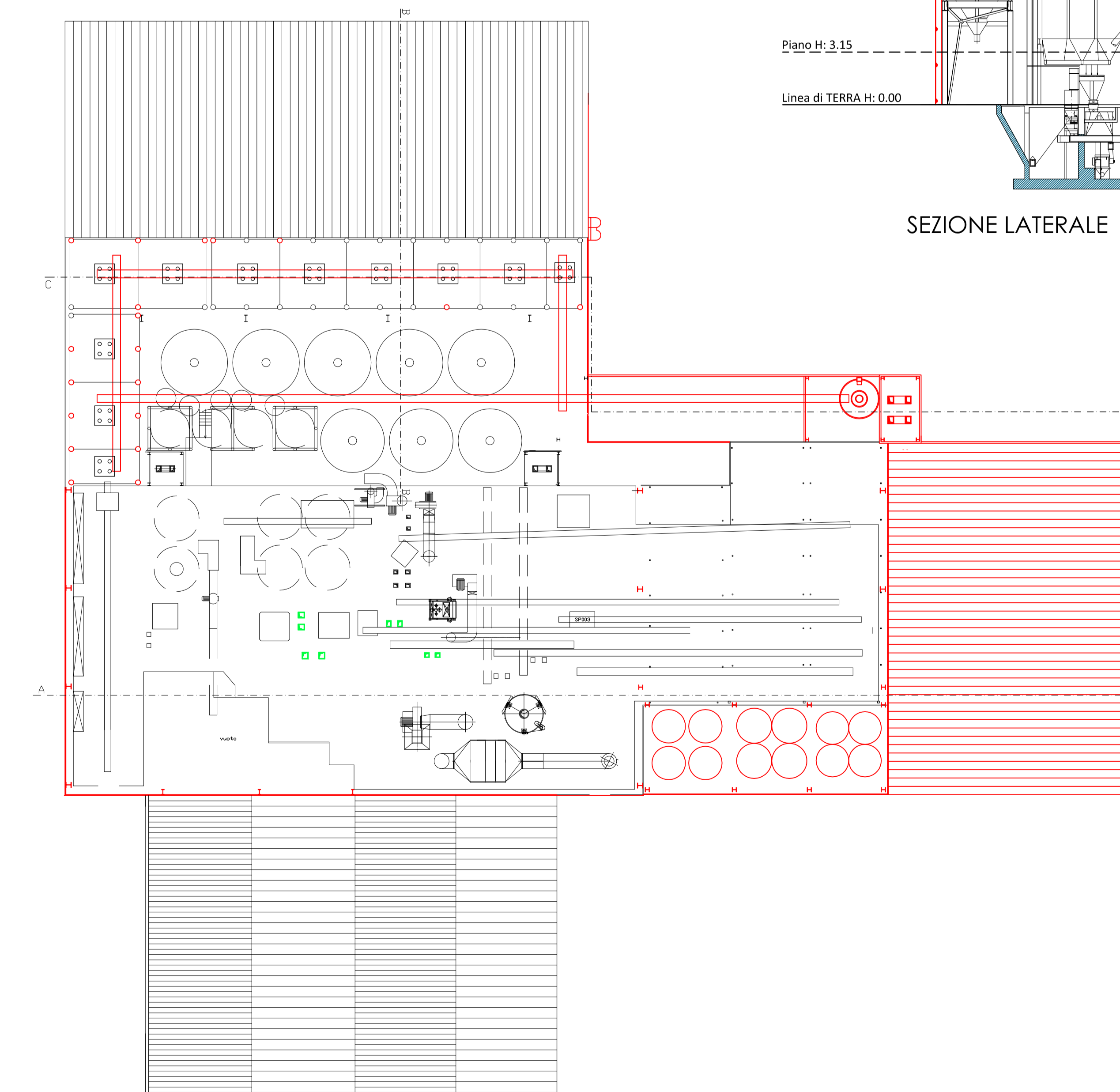
Piano H: 26.00 scala 1:100
